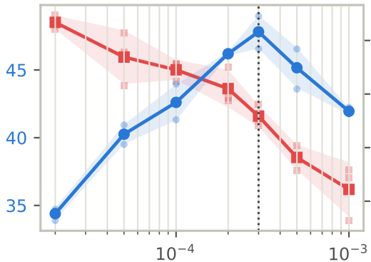
CLoRA
