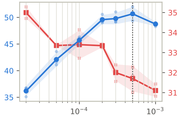
SC-LoRA
